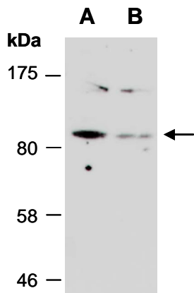
Fig 1. Western blot of total cell extracts from A) human HeLa, B) human Jurkat; using anti-ZBTB16 (C) (R0075-4a) at RT for 2 h.
